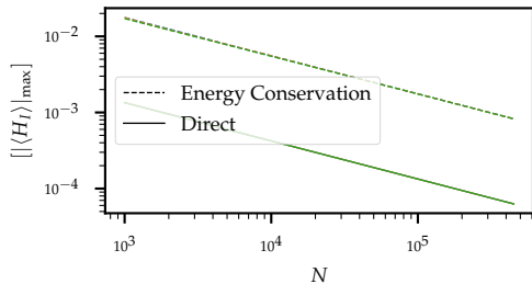
Statistical Error of \langle H_I \rangle .
