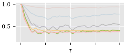
\omega_c = 1 , Estimates \in [0.02, 0.44]
