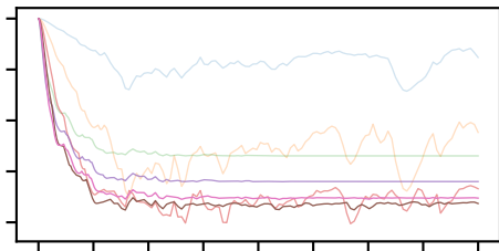
\omega_c = 4 , Estimates \in [0.01, 0.22]
