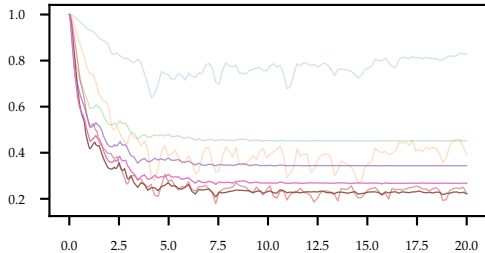
\omega_c = 3 , Estimates \in [0.01, 0.26]
