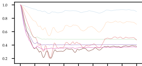
\omega_c = 3 , Estimates \in [0.01, 0.26]
