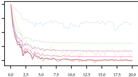
\omega_c = 4 , Estimates \in [0.01, 0.22]
