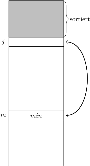
Selectionsort
