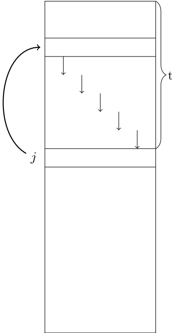
Insertionsort
